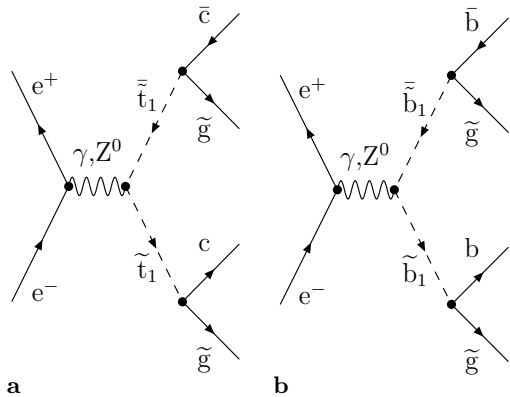
Fig. 2a,b. Stop a and sbottom b production and decay at LEP2
