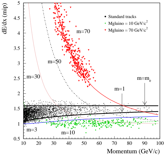
Fig. 6. The lines show the theoretical ionization energy loss as a function of the momentum of the particle for different mass cases ( \text{GeV}/c^2 ). The black points are reconstructed tracks coming from Z^0 \rightarrow q\bar{q} events generated at \sqrt{s} = 200 GeV, while the stars and the triangles correspond to R^\pm tracks with mass of 10 and 70 \text{GeV}/c^2 respectively. The dE/dx is expressed in units of energy loss for a minimum ionizing particle
