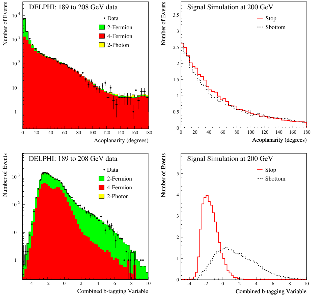
Fig. 14. Data-simulation comparison at the preselection level of the LEP2 q\bar{q}R^{\circ}R^{\circ} analysis. Data taken in the centre-of-mass energy range between 189 and 208 GeV were included. Right-hand side histograms show the expected distributions with arbitrary normalization for the stop and the sbottom signal at 200 GeV when all simulated samples are added together
