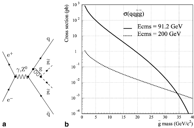
Fig. 1. a Gluon splitting into a pair of gluinos. b Comparison of the cross-section (pb) of this process at centre-of-mass energies of 91.2 GeV (LEP1) and of 200 GeV (LEP2)
