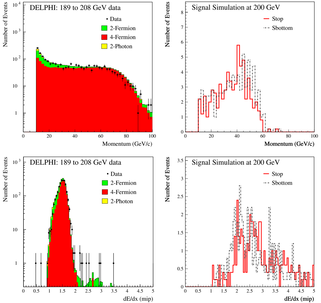
Fig. 11. Momentum and dE/dx of the charged R -hadron candidates selected by the q\bar{q}R^\pm R^0 analysis at LEP2. Data taken in the centre-of-mass energy range between 189 and 208 GeV were included. Right-hand side histograms show the expected distributions for one possible stop and sbottom signal ( m_{\tilde{q}_1} = 90 \text{ GeV}/c^2 , m_{\tilde{g}} = 60 \text{ GeV}/c^2 ) at \sqrt{s} = 200 \text{ GeV} with arbitrary normalization
