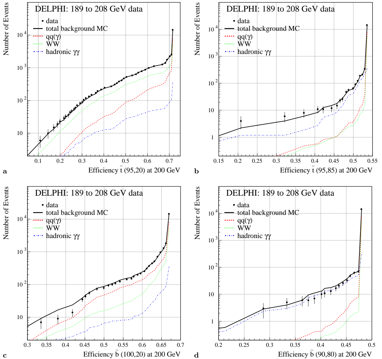
Fig. 15a–d. Numbers of events as a function of the signal efficiencies for the stop and sbottom analysis. Data taken in the centre-of-mass energy range between 189 and 208 GeV were included. a stop analysis for \Delta m > 20 \text{ GeV}/c^2 and b for \Delta m \leq 20 \text{ GeV}/c^2 , c sbottom analysis for \Delta m > 20 \text{ GeV}/c^2 and d for \Delta m \leq 20 \text{ GeV}/c^2 . The squark and gluino mass values used for the signal detection efficiencies are indicated on the x axis, (m_{\tilde{q}_1}, m_{\tilde{g}})
