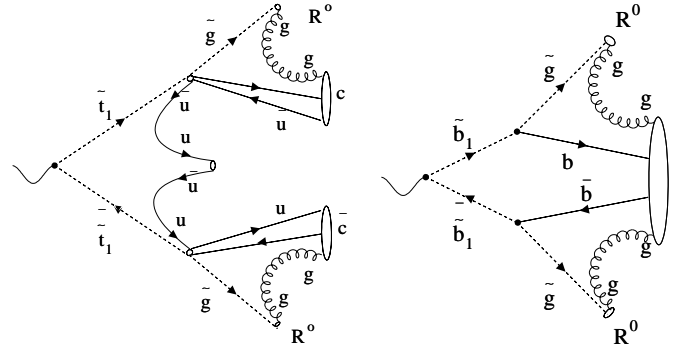
Fig. 3. Production and decay of the stop and sbottom squarks. Ellipses indicate the color singlet and the color string stretched between the partons
