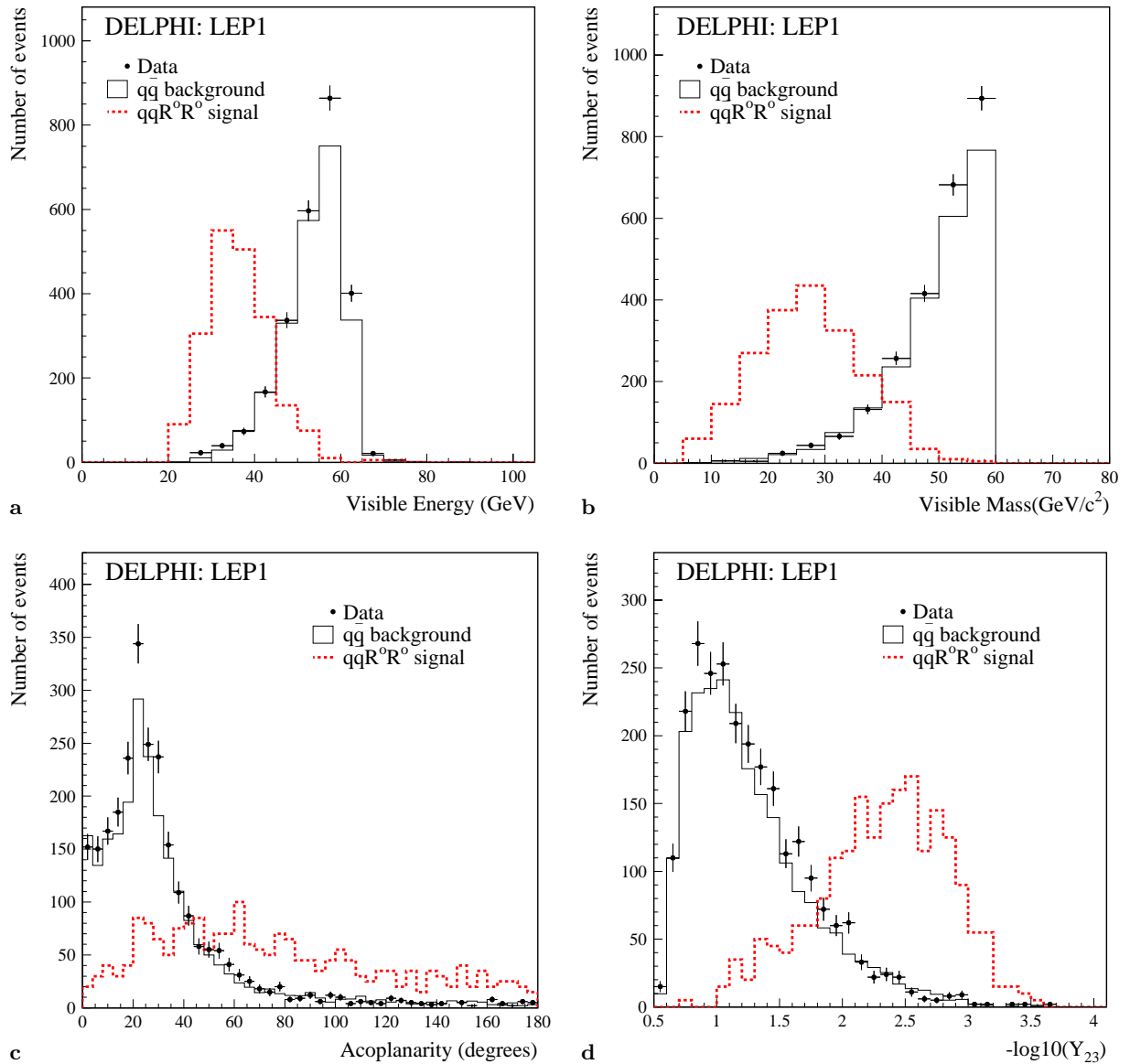
Fig. 8a–d. Comparison between data and simulation in the q\bar{q}R^0R^0 analysis at LEP1. a visible energy, b visible mass, c acoplanarity d DURHAM distance Y_{23} . Dotted lines show the q\bar{q}R^0R^0 signal distributions with arbitrary normalization when all simulated samples are added together
