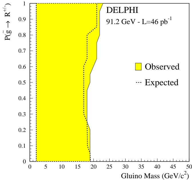
Fig. 17. Results of the LEP1 analysis: excluded region at 95% confidence level in the plane (m_{\tilde{g}}, P) . P is the probability that the gluino hadronizes to a charged R-hadron. The shaded region corresponds to the observed exclusion and the line to the expected one
