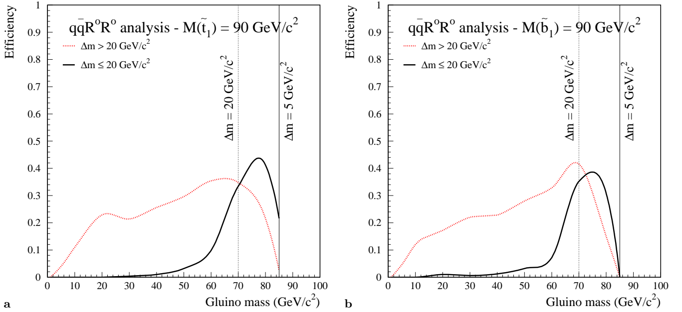
Fig. 16a,b. Signal detection efficiencies at \sqrt{s} = 200 GeV for the stop a and sbottom b q\bar{q}R^{\circ}R^{\circ} analysis as a function of the gluino mass ( m_{\tilde{q}_1} = 90 \text{ GeV}/c^2 )
