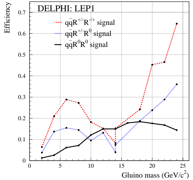
Fig. 7. Signal detection efficiencies in the LEP1 data analyses as a function of the gluino mass for the three signal topologies q\bar{q}R^\pm R^\pm , q\bar{q}R^\pm R^0 and q\bar{q}R^0 R^0 . The search for charged R-hadrons was optimized separately for low gluino masses ( < 14 \text{ GeV}/c^2 ) and for high gluino masses ( \geq 14 \text{ GeV}/c^2 )
