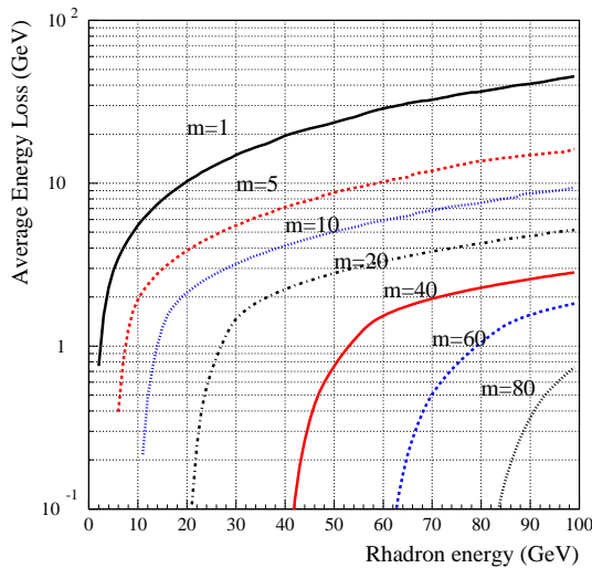
Fig. 4. Average energy loss by neutral R-hadrons in the DELPHI calorimeters as a function of their initial energy for different mass cases
