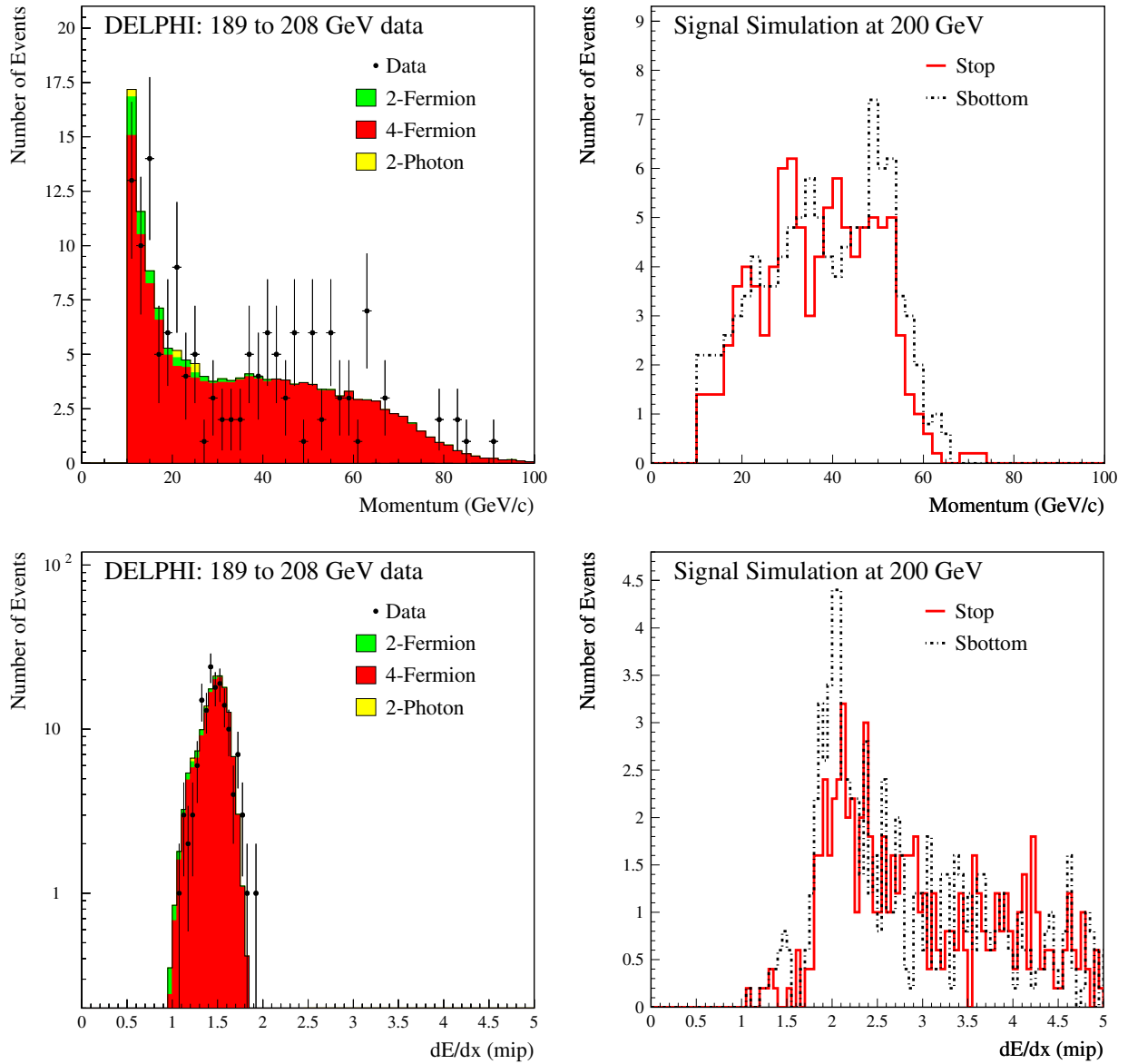
Fig. 9. Momentum and dE/dx of the charged R-hadron candidates selected by the q\bar{q}R^{\pm}R^{\pm} analysis at LEP2. Data taken in the centre-of-mass energy range between 189 and 208 GeV were included. Right-hand side histograms show the expected distributions for one possible stop and sbottom signal ( m_{\tilde{q}_1} = 90 \text{ GeV}/c^2 , m_{\tilde{g}} = 60 \text{ GeV}/c^2 ) at \sqrt{s} = 200 \text{ GeV} with arbitrary normalization
