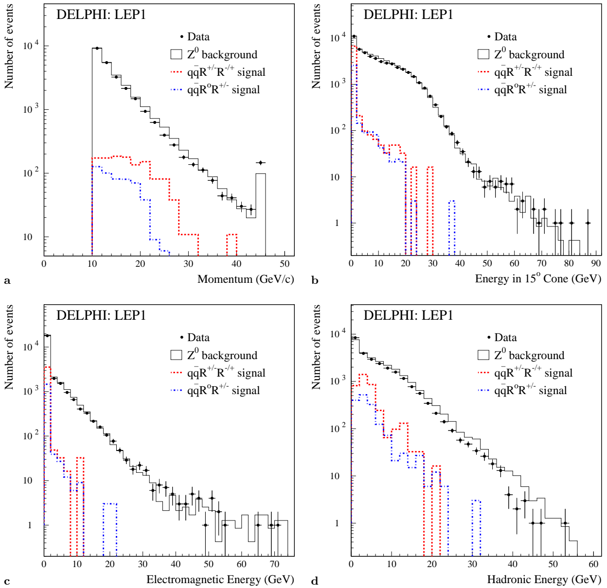
Fig. 5a–d. Comparison between data and simulation in the search for charged R-hadrons at LEP1. The plots show characteristic distributions before the selection of the charged R-hadron candidates: a the momentum, b the total energy in a 15° degree cone around the particle, c its electromagnetic and d hadronic energy. Dotted lines show the qqR^{\pm}R^{\pm} and qqR^{\pm}R^0 signal distributions with arbitrary normalization when all simulated samples are added together
