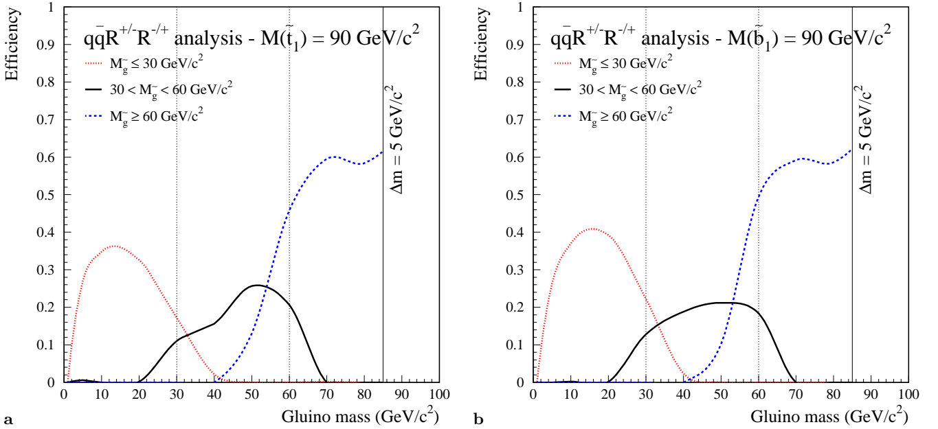
Fig. 10a,b. Signal detection efficiencies at \sqrt{s}=200 GeV for the stop a and sbottom b q\bar{q}R^{\pm}R^{\pm} analysis as a function of the gluino mass ( m_{\tilde{q}_1} = 90 GeV/c 2 ). \Delta M is the mass difference between the squark and the gluino. Vertical lines show the limits of the mass analysis window. The last one ends at \Delta M = 5 GeV/c 2 which corresponds the last simulated signal points
